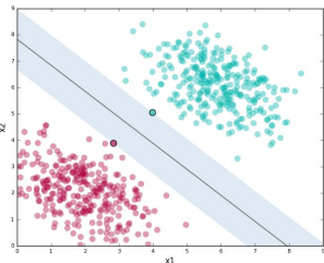
Machine Learning
