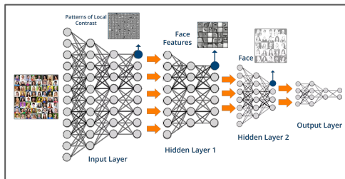
Deep Learning
