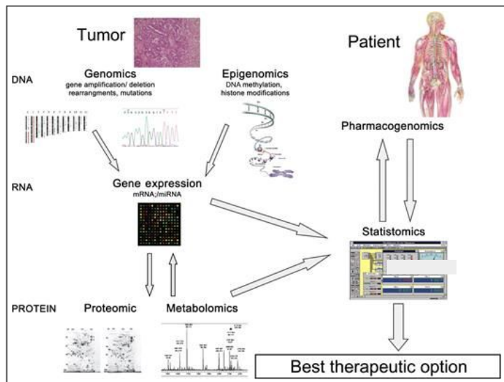
Machine Learning
